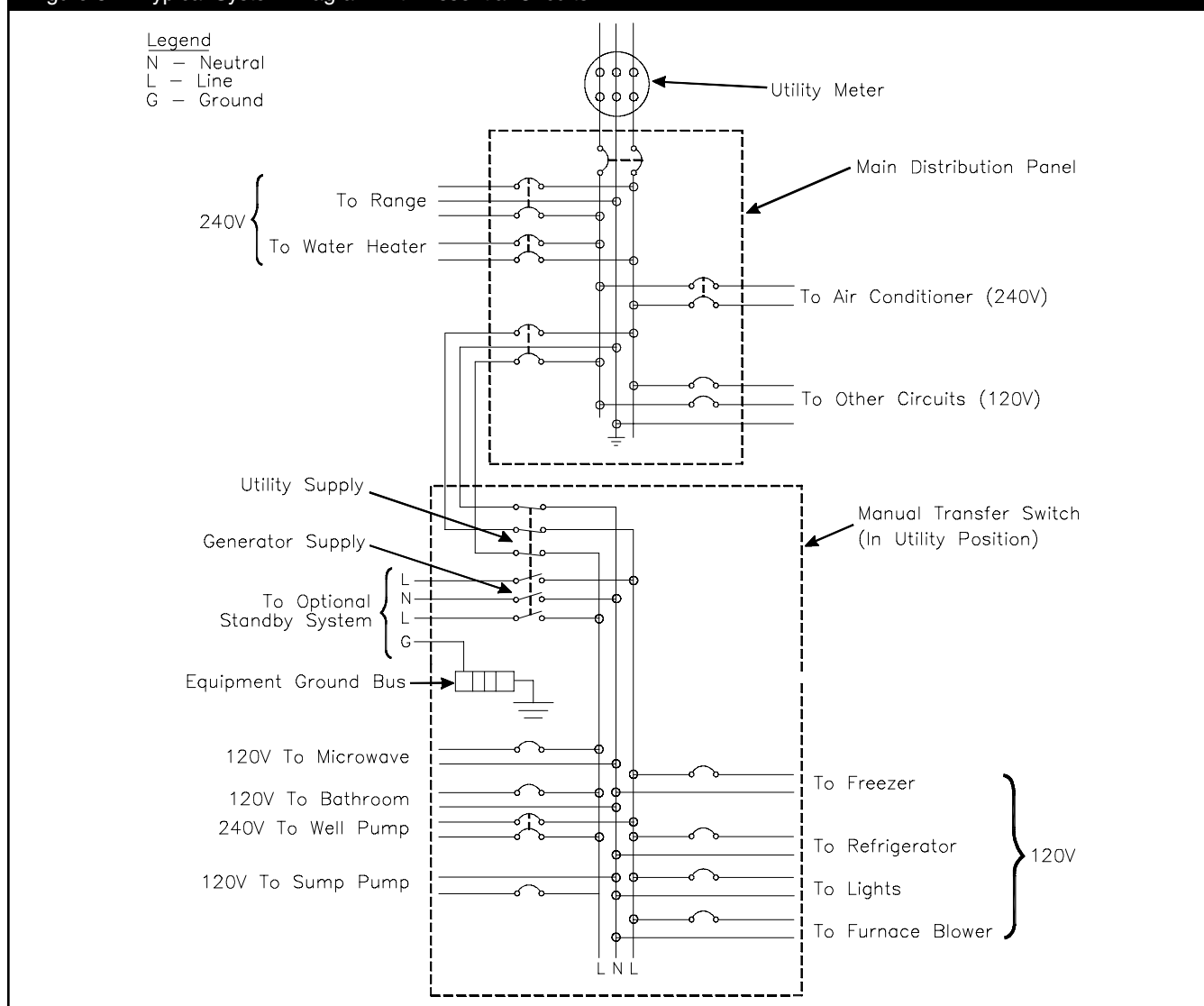
Figure 3 — Typical System Diagram with Essential Circuits
