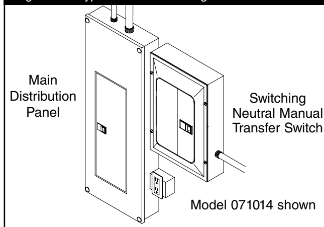
Figure 2 — Typical Switch Mounting
